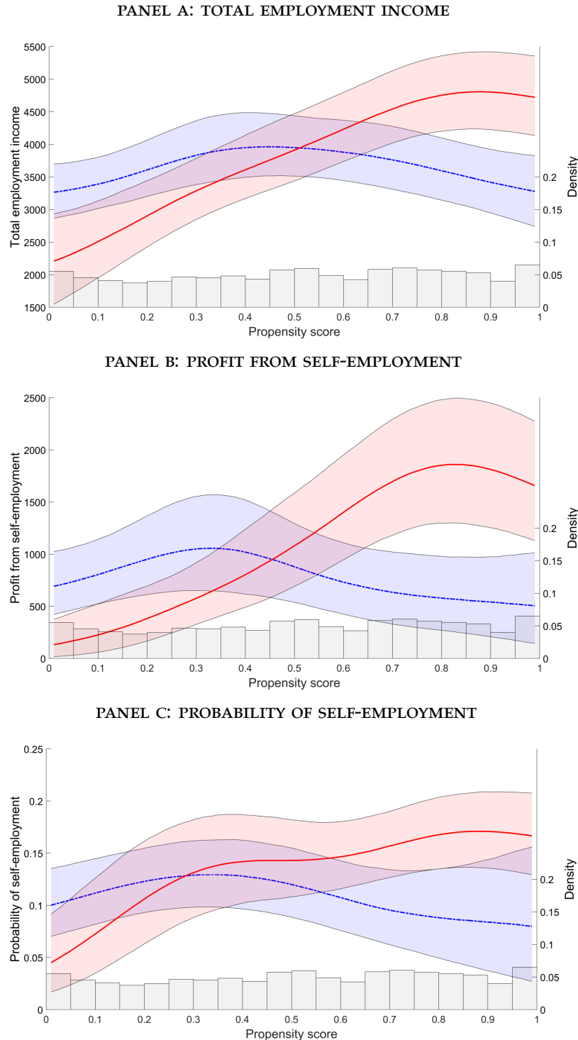
Figure 4: Treatment heterogeneity under matching
