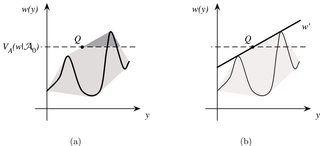
Figure 1: Sketch of the main proof: (a) Identifying the worst-case point for a given contract w(y) . (b) Improving w to an affine contract w' .
