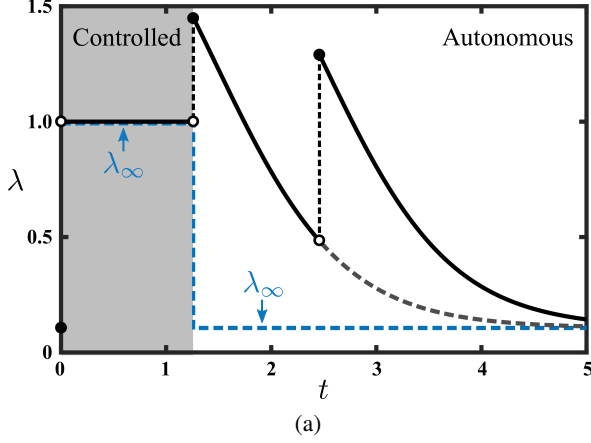
Figure C2: Numerical illustration: (a) Bayesian intensity dynamics; (b) Autonomous and controlled parameters.
