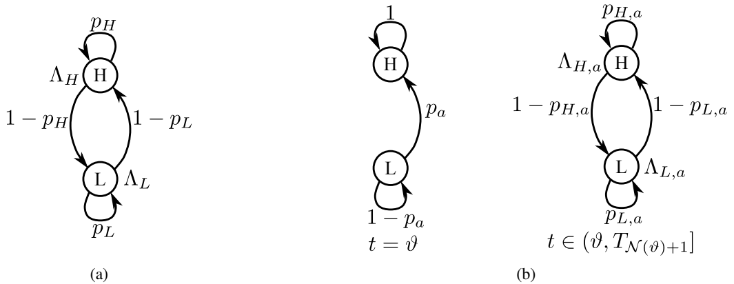
Figure C1: (a): Binary Markov jump process; (b): controlled Markov jump process.
