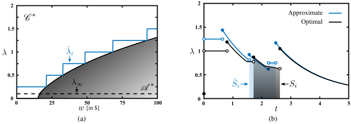
Figure D1: Approximation of the optimal collection strategy A^* by an \mathcal{M} -envelope strategy A_{\mathcal{M}}^* , (a): in the (intensity, balance)-space; (b): in the time domain (where \tilde{S}_i = S_i are i.i.d. exponential).
