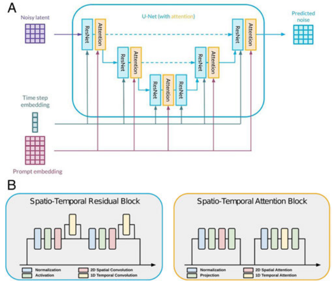
Figure 5: Denoising U-Net with Spatio-temporal Attention. (A) Common attention U-Net used for the denoising step in image and video diffusion models comprising residual convolution blocks and attention blocks as well as concatenated time step and text prompt-embeddings. Figure adapted from [KDS23]. (B) Temporal structure in video diffusion and editing is commonly modeled by adding 1D temporal convolutions in the residual blocks (left) as well as 1D temporal attention blocks after each of the 2D spatial attention blocks (right). Figure adapted from [ECA*23].
