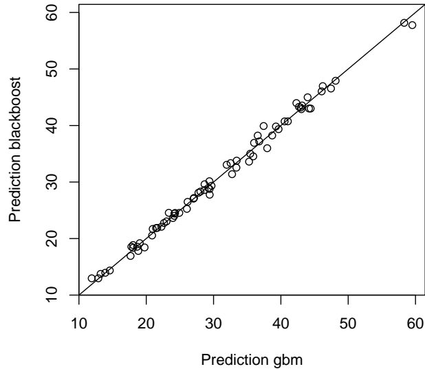
FIG 4. bodyfat data: Fitted values of both the gbm and mboost implementations of L_2 Boosting with different regression trees as base learners.
