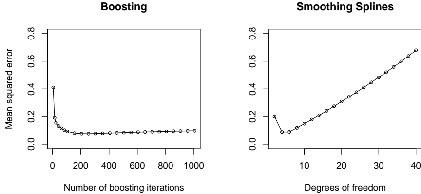
FIG 5. Mean squared prediction error \mathbb{E}[(f(X) - \hat{f}(X))^2] for the regression model Y_i = 0.8X_i + \sin(6X_i) + \varepsilon_i ( i = 1, \dots, n = 100 ), with \varepsilon \sim \mathcal{N}(0, 2) , X_i \sim \mathcal{U}(-1/2, 1/2) , averaged over 100 simulation runs. Left: L_2 Boosting with smoothing spline base procedure (having fixed degrees of freedom df = 4 ) and using \nu = 0.1 , for varying number of boosting iterations. Right: single smoothing spline with varying degrees of freedom.
