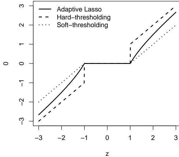
FIG 8. Hard-threshold (dotted-dashed), soft-threshold (dotted) and adaptive Lasso (solid) estimator in a linear model with orthonormal design. For this design, the adaptive Lasso coincides with the non-negative garrote [13]. The value on the x-axis, denoted by z , is a single component of \mathbf{X}^\top \mathbf{Y} .
