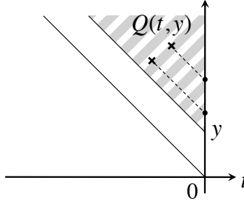
Figure 2: The points lies in the shaded area correspond to people who are still in the system at time 0 with remaining service time greater than y
