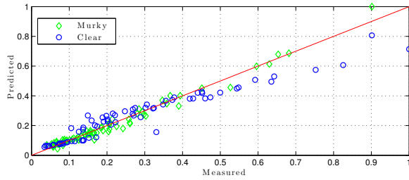
Fig. 4. Prediction scatter plot for data presented in Fig. 3
