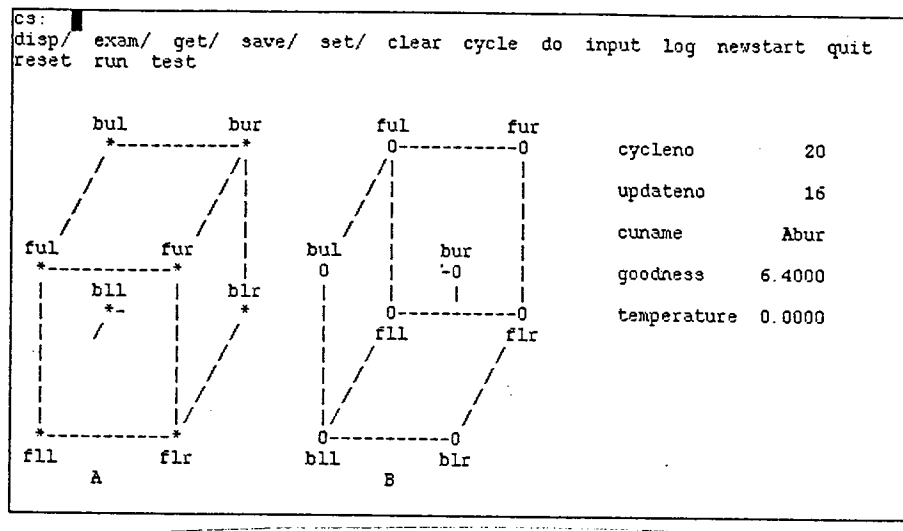
FIGURE 3. The state of the system after 20 cycles.
