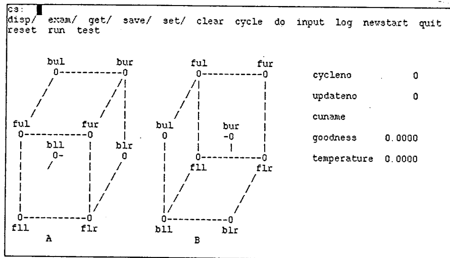
FIGURE 2. The initial image of the screen for the cube example.
