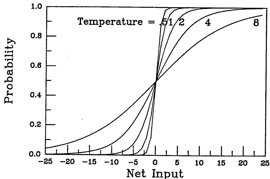
FIGURE 7. Activation probabilities according to the logistic function. (From PDP-2 , p. 69.)
