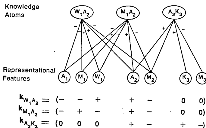
FIGURE 8. The graphical representation of a particular harmony model. In this model, the representational features represent letters in particular positions, and the knowledge atoms represent common letter combinations. (From PDP-6 , p. 216.)
