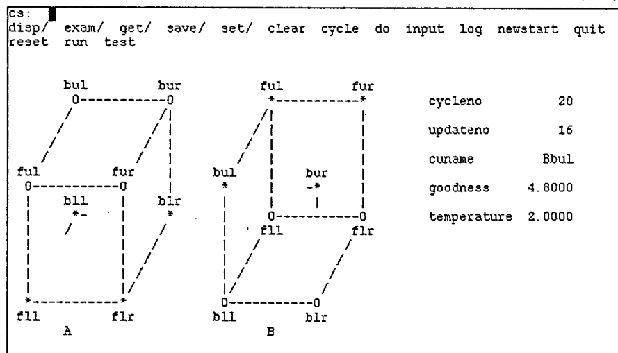
FIGURE 6. A local minimum with the Necker cube.
