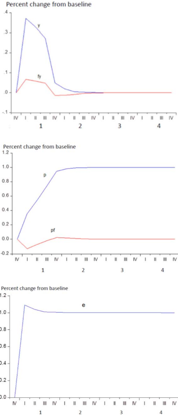
Figure 2: Small International Monetary Spillovers in a Two-Country Model. Simulation of an unanticipated permanent 1% increase in the money supply in one country in two-country model, showing impact on output and price level relative to the baseline in Country 1 ( y and p ) and in Country 2 ( y_f and p_f ), and the exchange rate ( e ).
