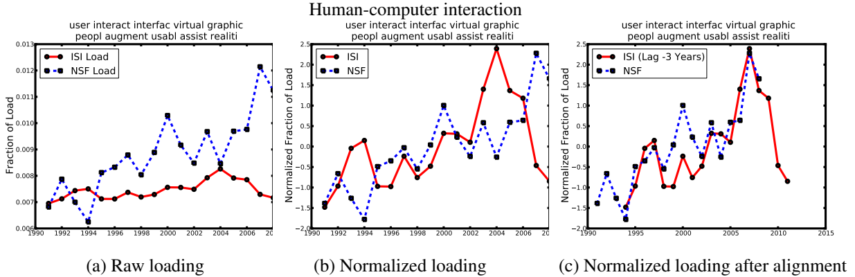
Figure 1: Estimation of lead/lag by aligning topic loadings.
