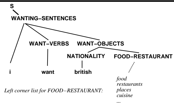
Figure 2: Prefixes and Left-Corner lists
