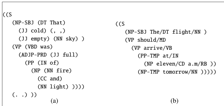
Figure F.7 Parsed sentences from the LDC Treebank3 version of the (a) Brown and (b) ATIS corpora.
