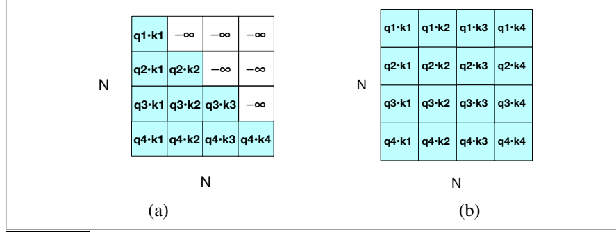
Figure 10.2 The N \times N \mathbf{QK}^T matrix showing the q_i \cdot k_j values. (a) shows the upper-triangle portion of the comparisons matrix zeroed out (set to -\infty , which the softmax will turn to zero), while (b) shows the unmasked version.
