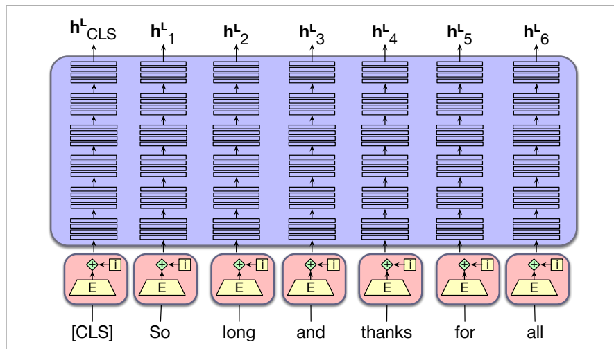
Figure 10.5 The output of a BERT-style model is a contextual embedding vector \mathbf{h}_i^L for each input token x_i .
