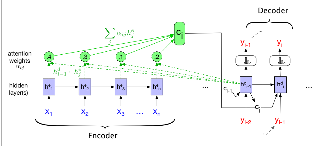
Figure 13.22 A sketch of the encoder-decoder network with attention, focusing on the computation of c_i . The context value c_i is one of the inputs to the computation of h^d_i . It is computed by taking the weighted sum of all the encoder hidden states, each weighted by their dot product with the prior decoder hidden state h^d_{i-1} .
