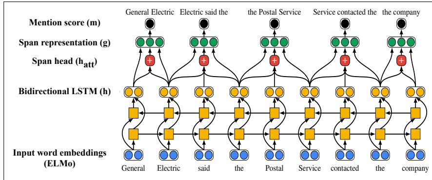
Figure 21.5 Computation of the span representation (using the biLSTM encoder) and the mention score in the end-to-end coreference model of Lee et al. (2017b). The model considers all spans up to a maximum width; the figure shows a small subset of these. Figure after Lee et al. (2017b).
