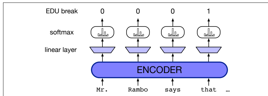
Figure 22.4 Predicting EDU segment beginnings from encoded text.
