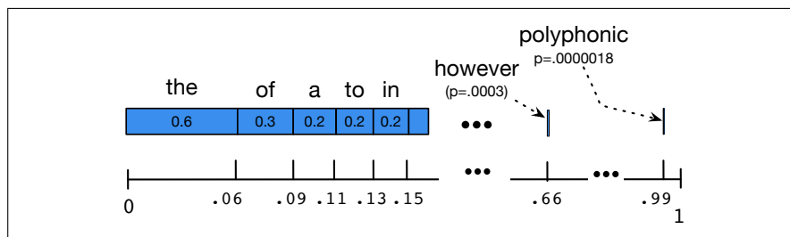
Figure 3.3 A visualization of the sampling distribution for sampling sentences by repeatedly sampling unigrams. The blue bar represents the frequency of each word. The number line shows the cumulative probabilities. If we choose a random number between 0 and 1, it will fall in an interval corresponding to some word. The expectation for the random number to fall in the larger intervals of one of the frequent words ( the , of , a ) is much higher than in the smaller interval of one of the rare words ( polyphonic ).
