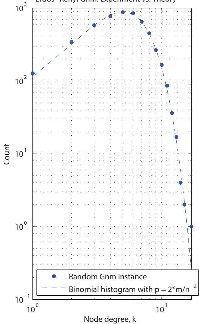
Erdos-Renyi Gnm: Experiment vs. Theory
