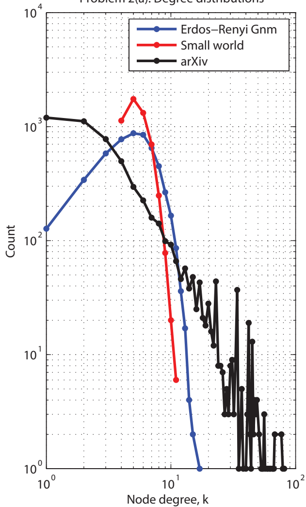
Problem 2(a): Degree distributions
