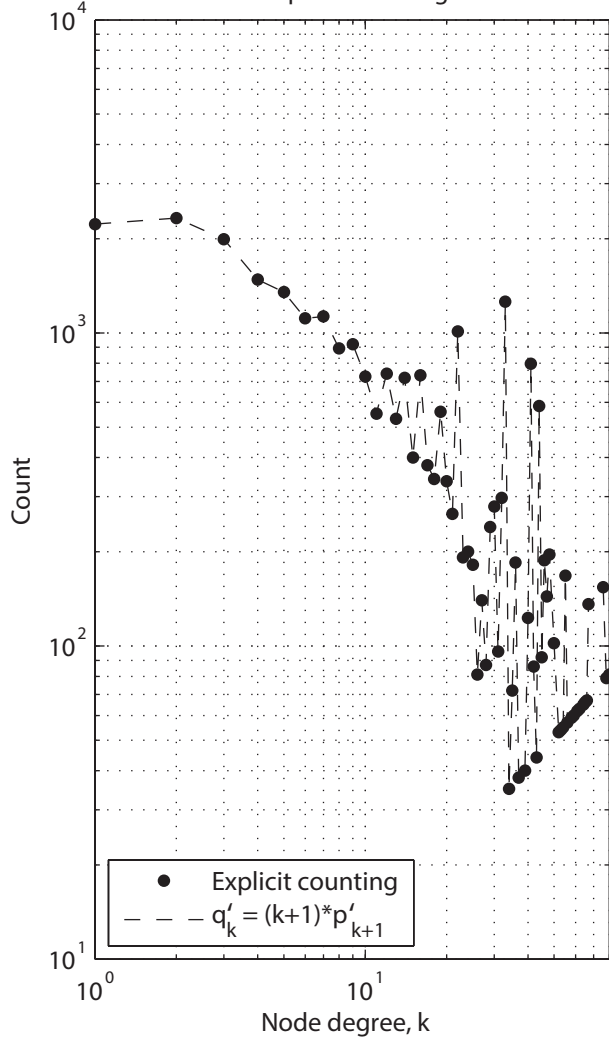
Excess distribution: explicit counting vs. closed-form
