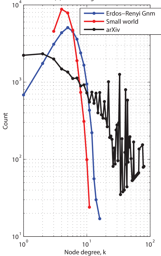
Problem 2(b): Excess degree distributions
