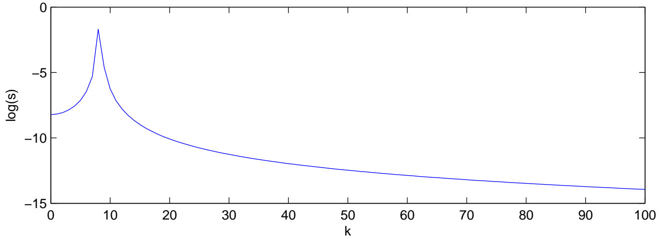
Power spectrum of theta for the above time series (first 8192 points used)
