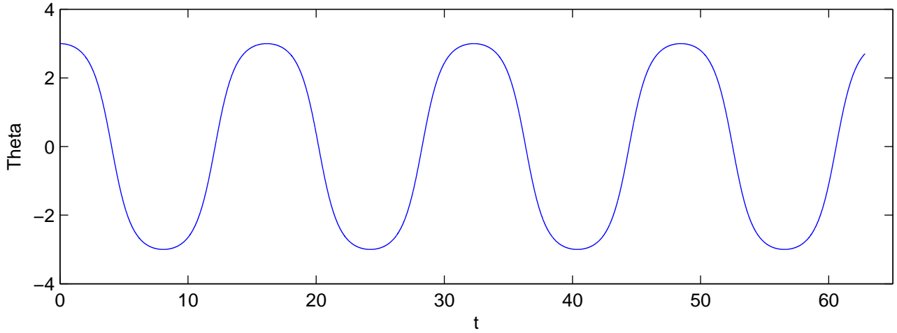
The undriven pendulum with IC = [3 0]
