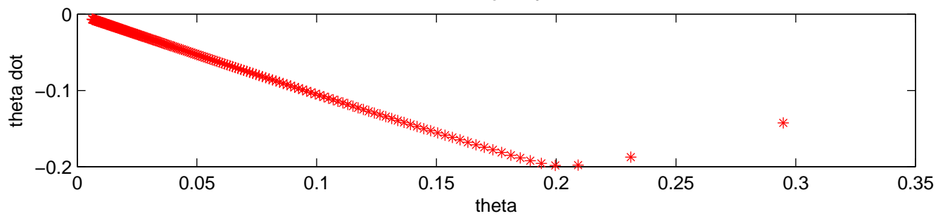
Poincare section sampled at w_s = w_0 = 1 (i.e. every 1000 units)
