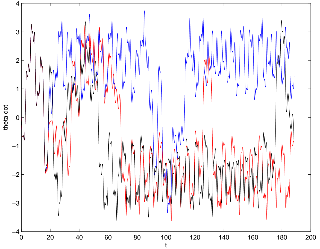
Sensitivity to initial conditions: IC(blue) = [0.5 0], IC(red) = [0.5001 0], IC(black) = [0.4999 0]
