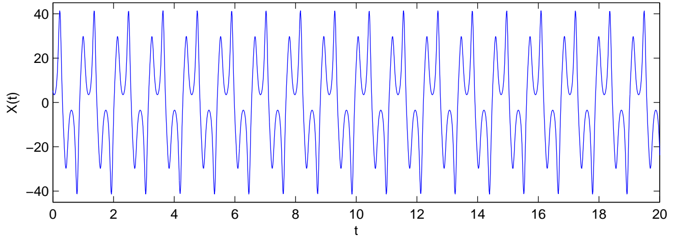
Steady state time series of Lorenz equation for r = 166 , b = 8/3
