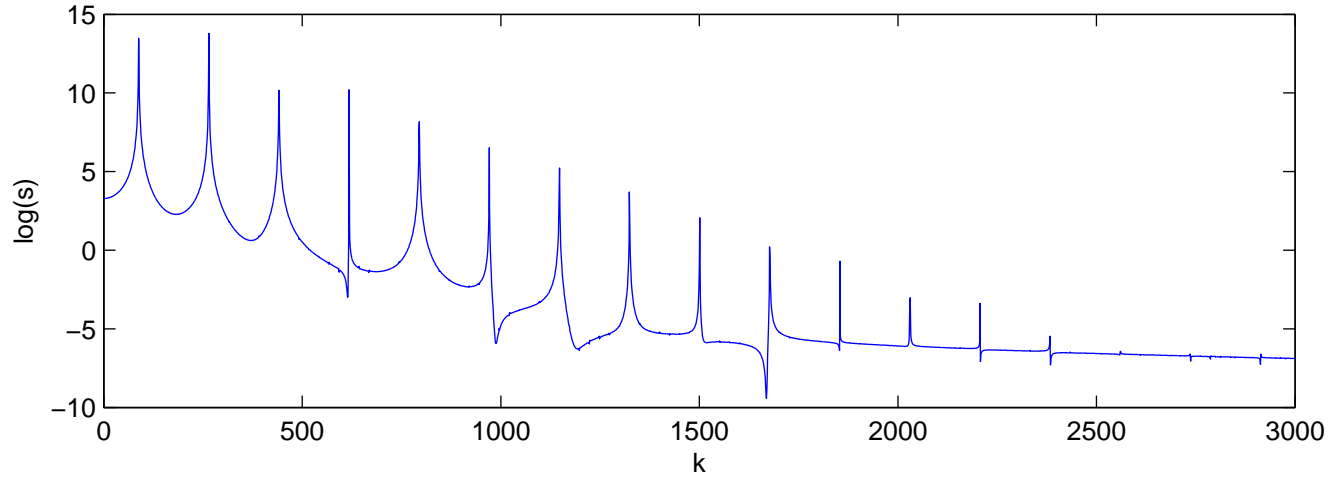
Power spectrum using tspan = 0:0.01:100
