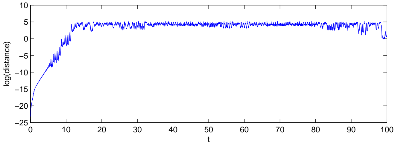
Separation between two trajectories over time for Lorenz system with r = 170 ; d_0 = 0.0000000001
