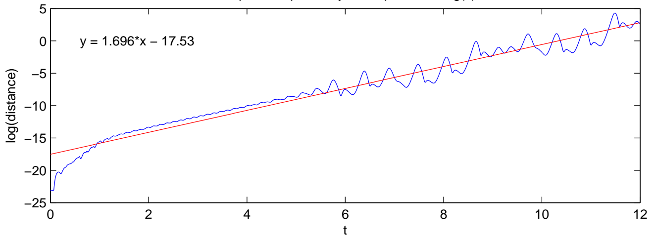
Close-up on the positively linear portion of \log(s) vs t
