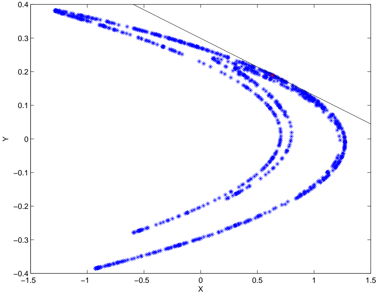
Problem 2: Henon map a=1.4 ; b=0.3
