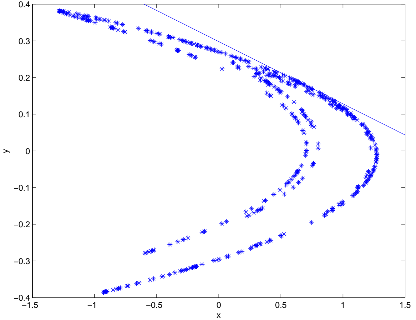
Henon map with y=-0.1697x+0.298 overlay
