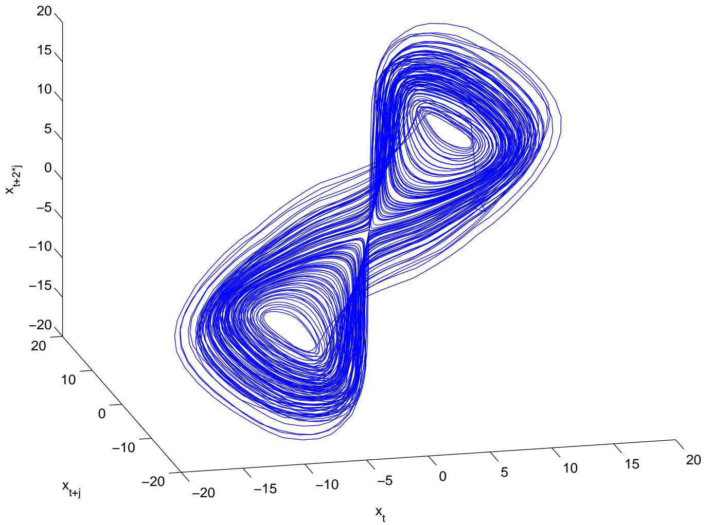
Phase space reconstruction from Lorenz X time series
