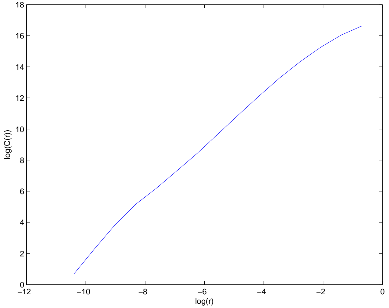
Correlation dimension curve for Lorenz X time series
