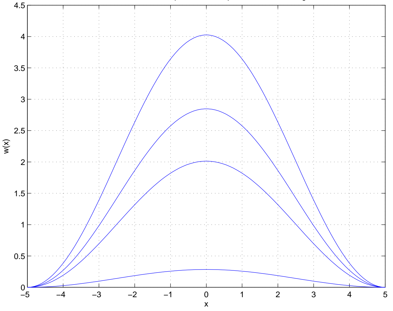
PS5, Problem 2: Compressed beam profile for several lengths
