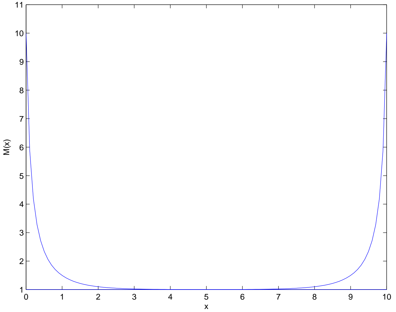
PS5, Problem 3: \nu = 1 . Boundary width: \sim 1
