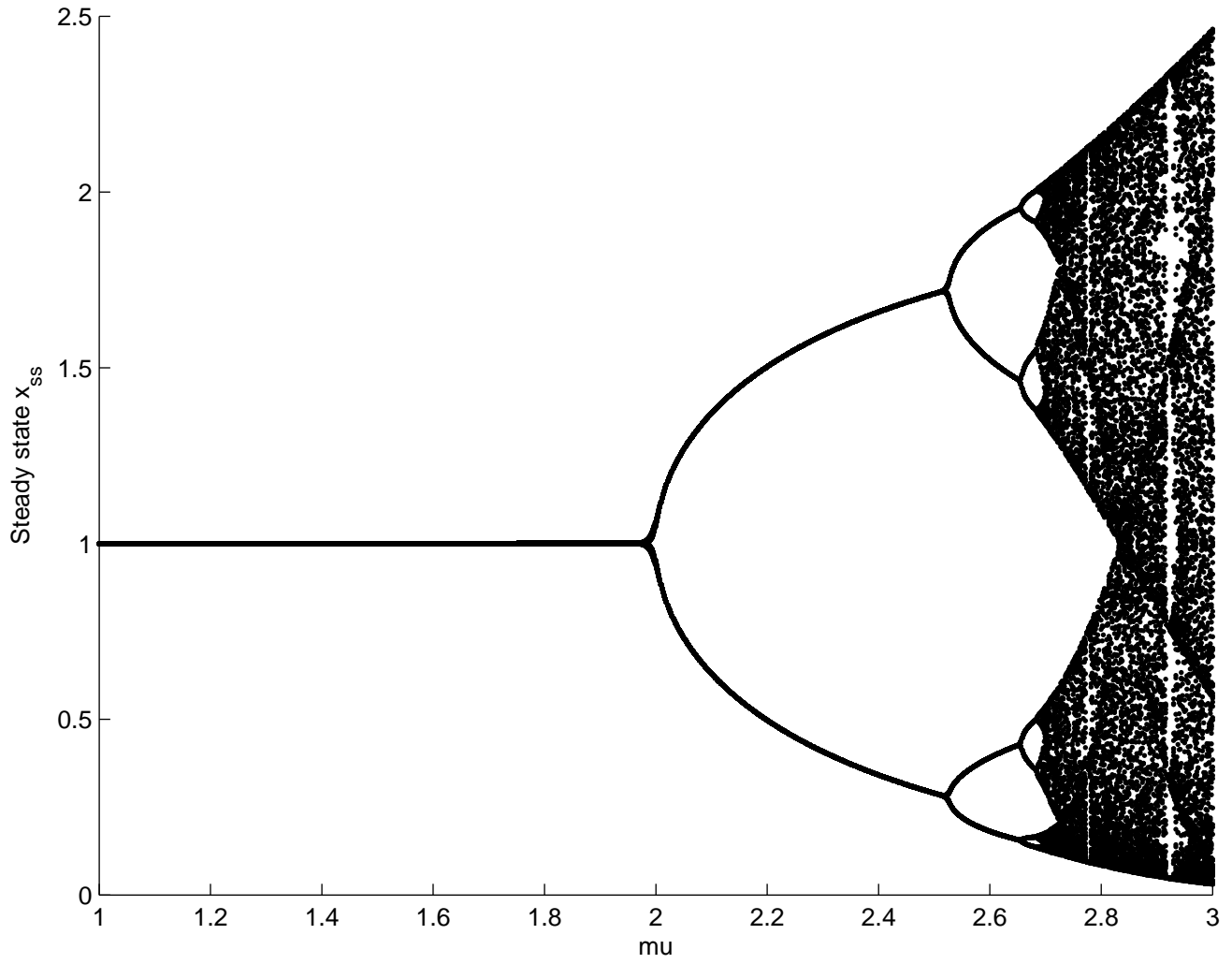
Bifurcation diagram for x_{n+1} = x_n * \exp(\mu * (1 - x_n))
