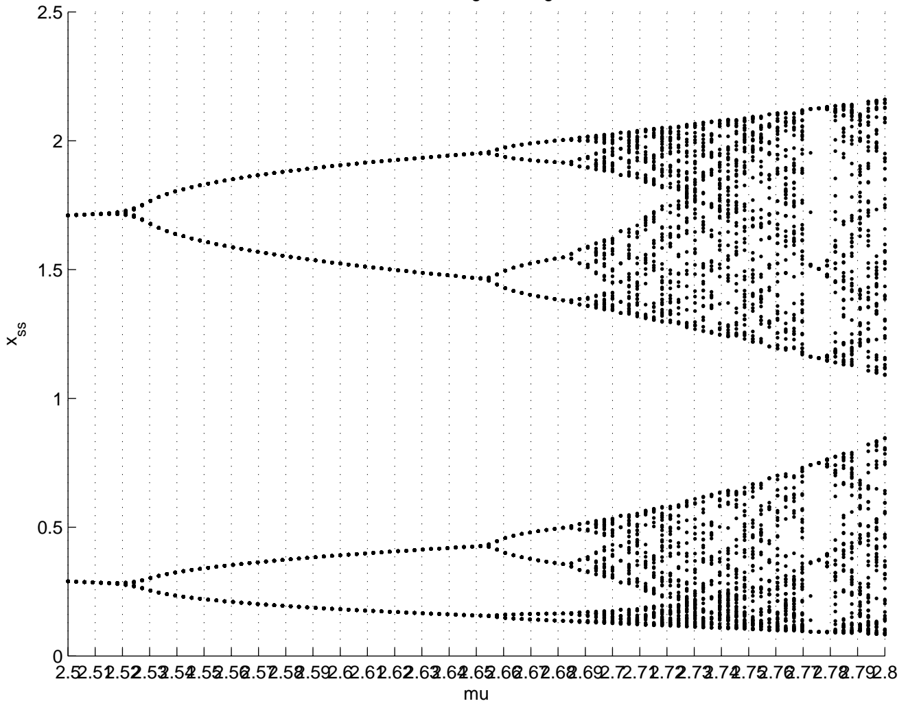
Bifurcation diagram magnified
