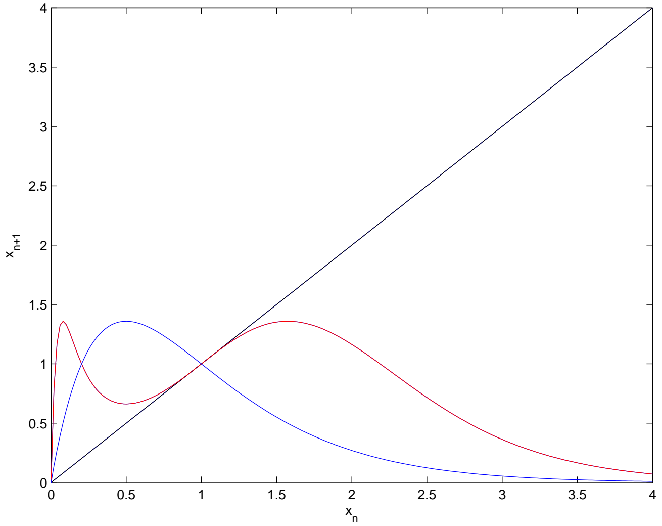
First and second return maps for x_{n+1} = x_n \exp(\mu(1-x_n)) ; \mu = 2
