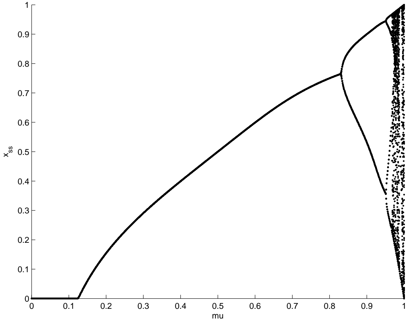
Bifurcation diagram for x_{n+1} = \mu \cdot (1 - (2 \cdot x_n - 1)^4)
