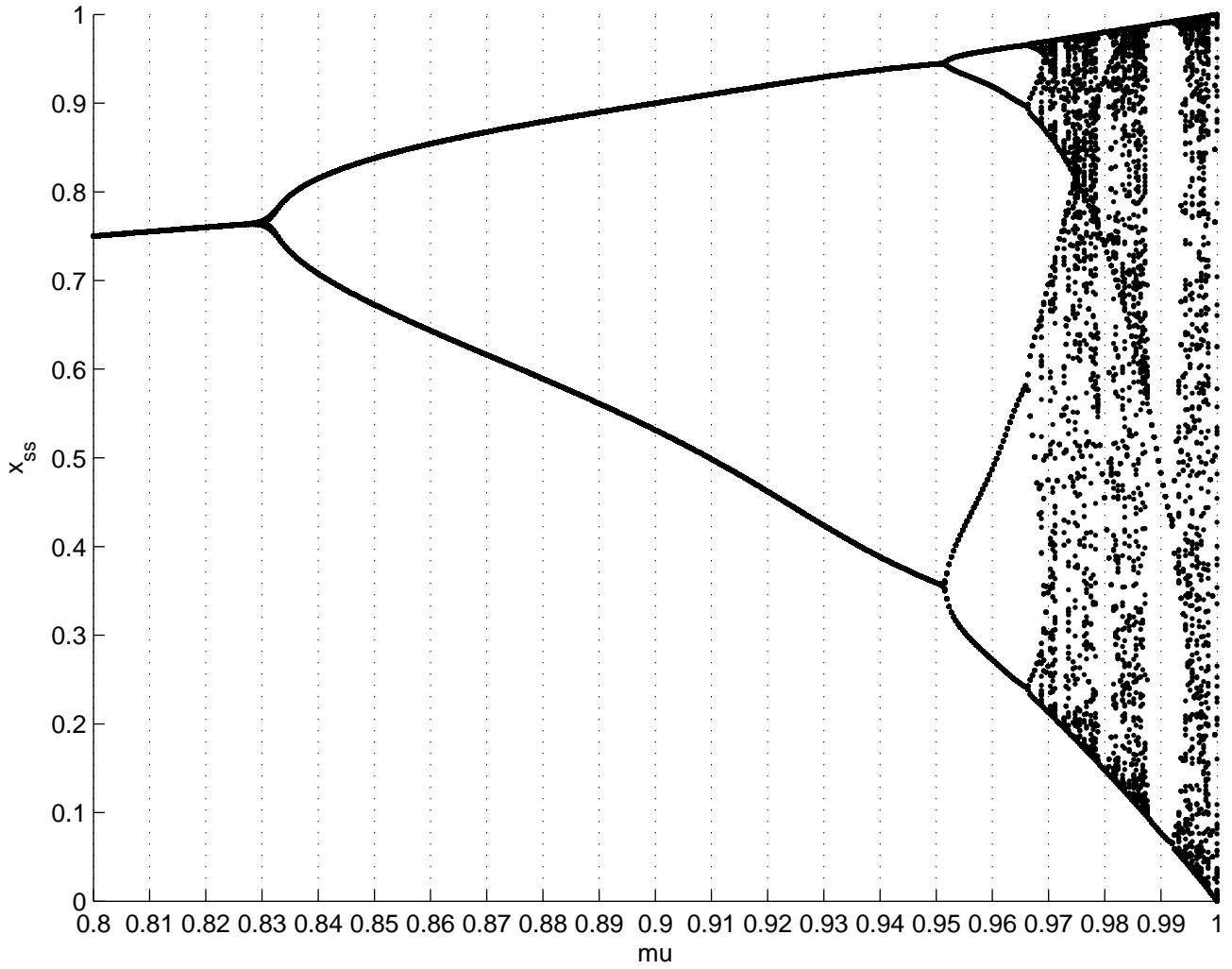
Magnified bifurcation diagram
