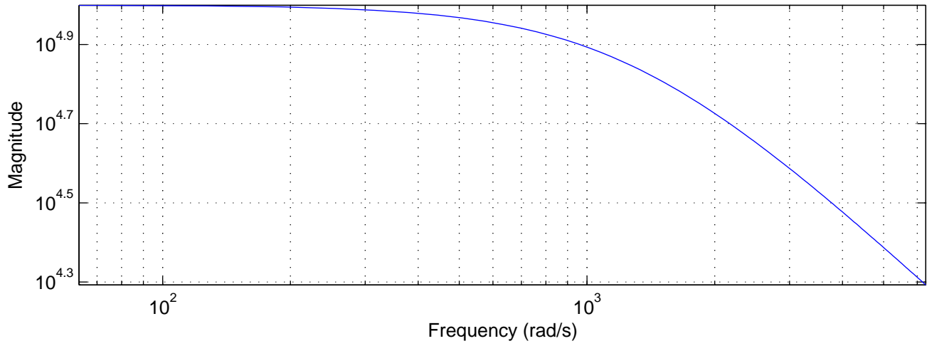
Frequency response of the simple opamp model
