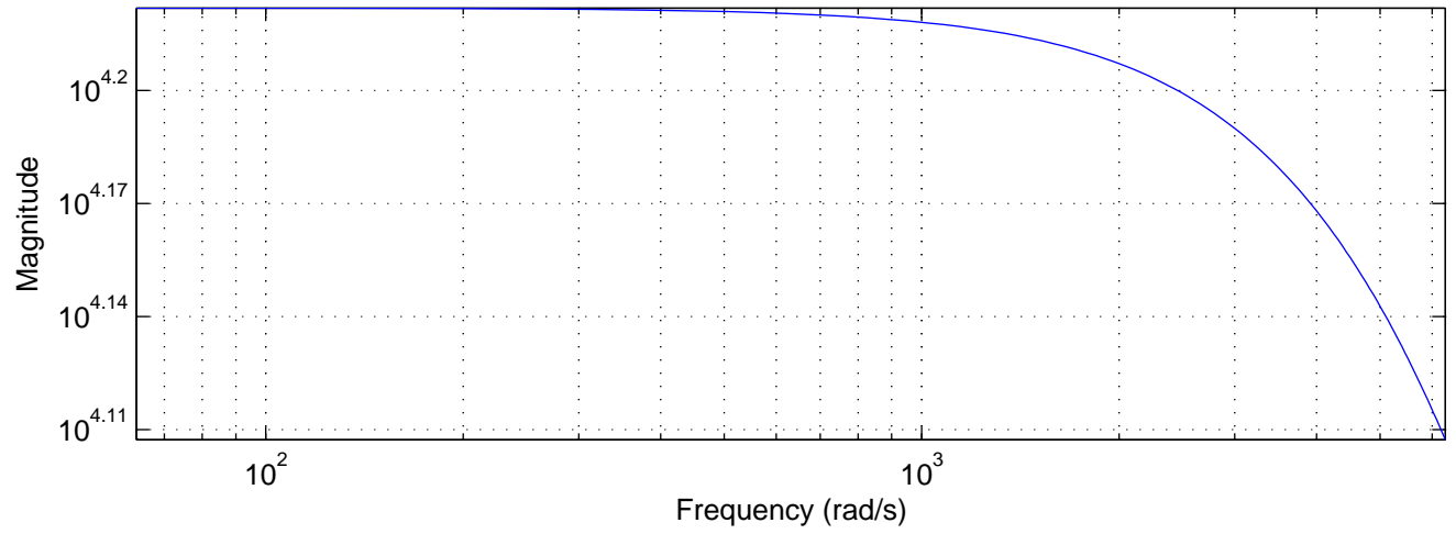
Frequency response of bandwidth-expanded opamp under feedback
