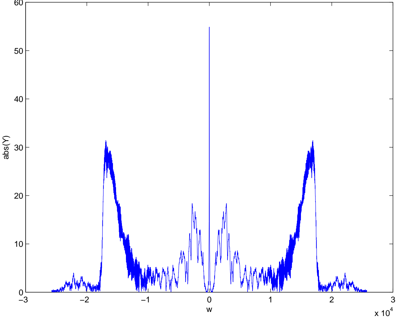
Part a: Fourier tranform of the sound file "splat"
