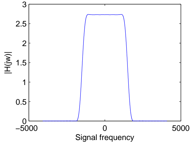
Part (d): Transform of ideal filter response
