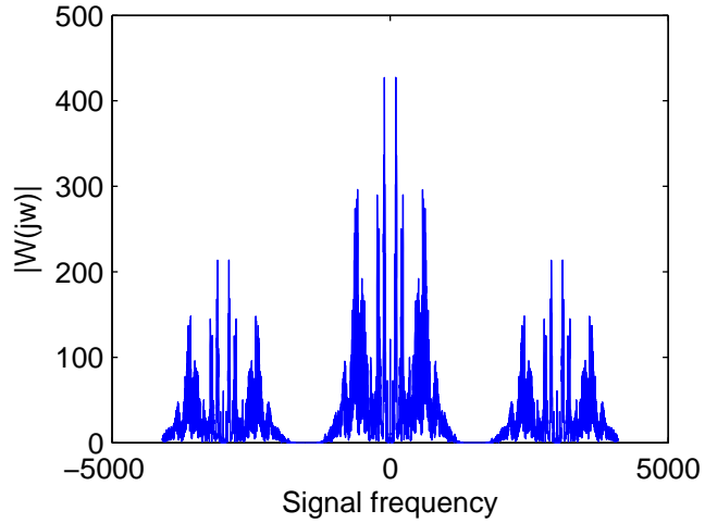
Part (c): The demodulated carrier
