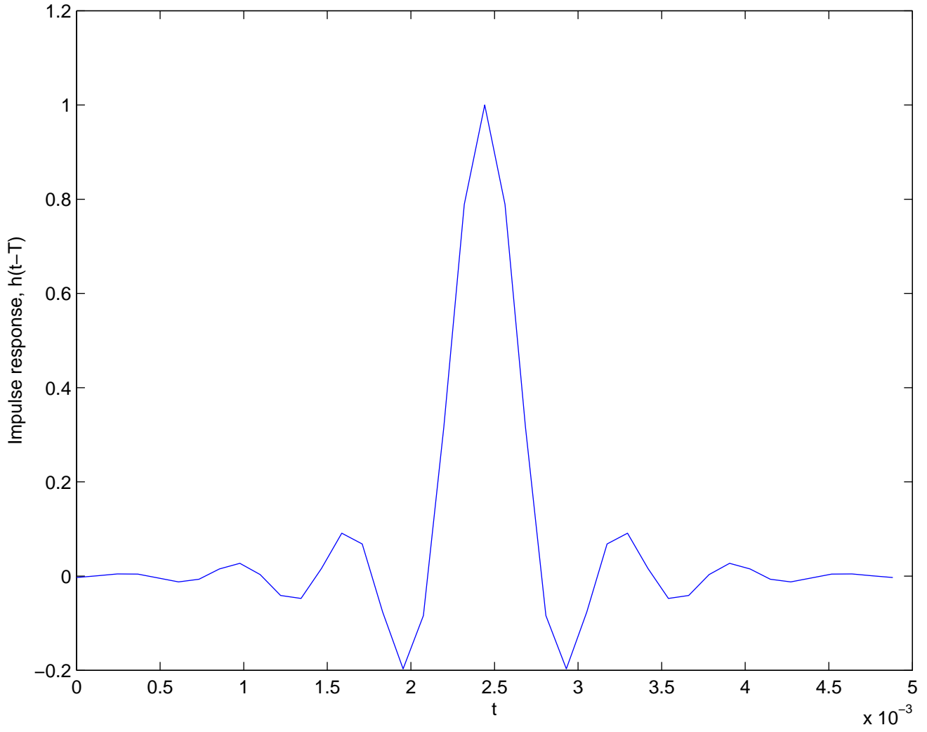
Part (d): Impulse response of ideal filter
