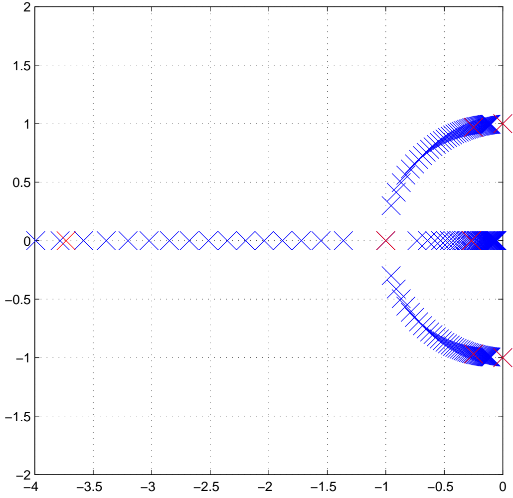
Trajectory of poles as \zeta is varied
