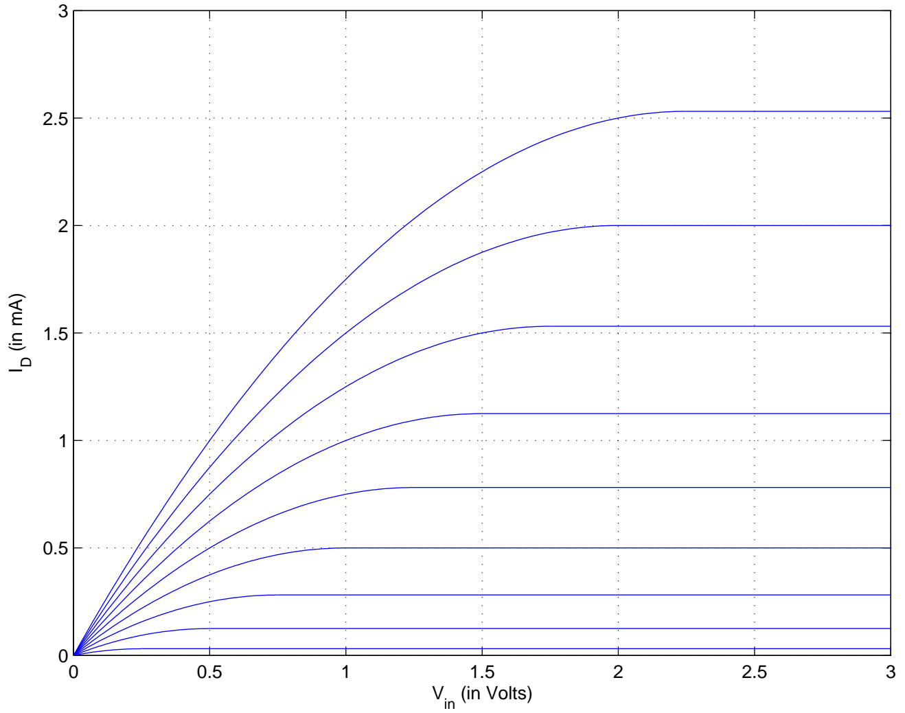
Problem 3, part (a): Output characteristics of pull-down transistor
