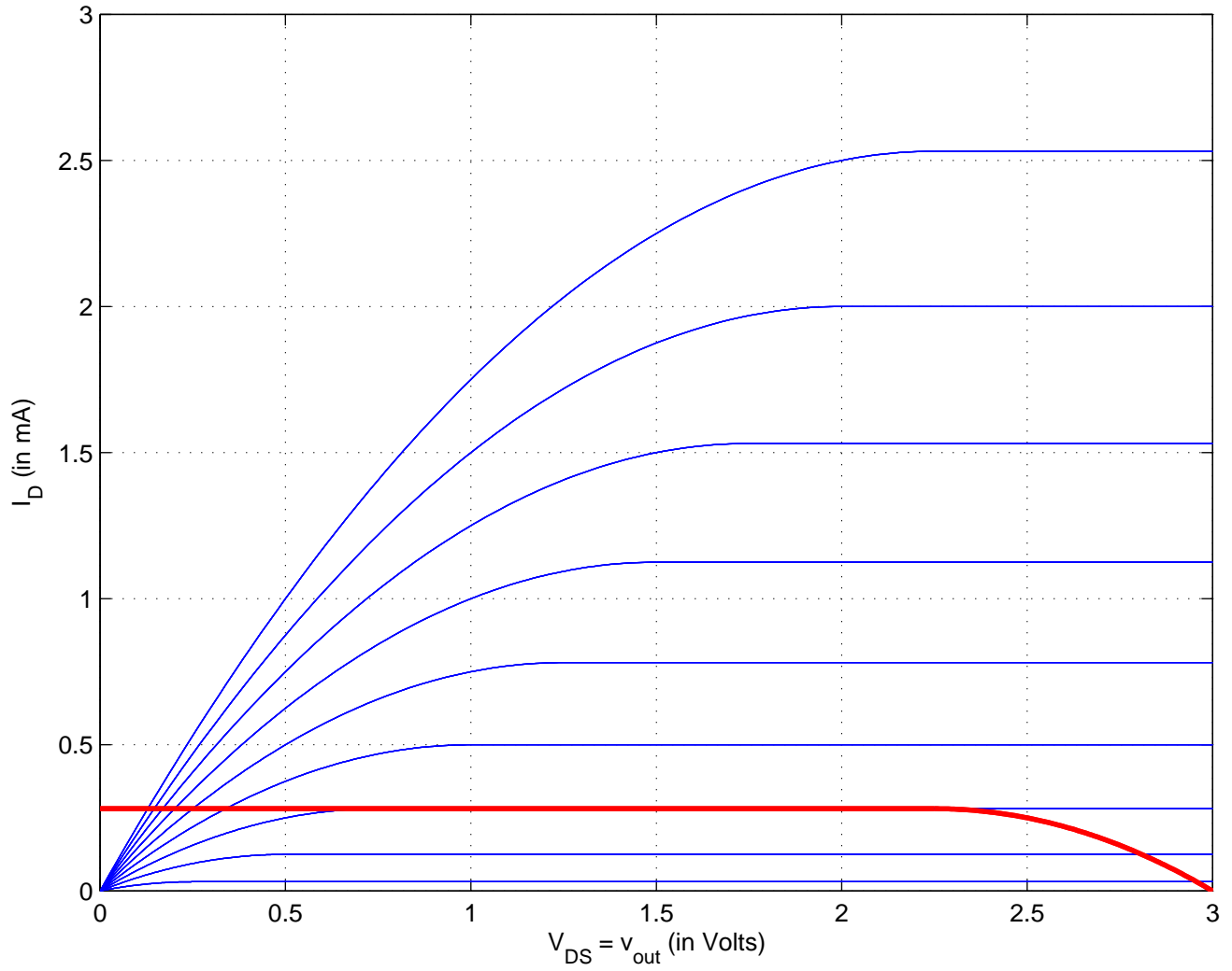
Problem 3, part (b): Load-line of pullup MOSFET included in red
