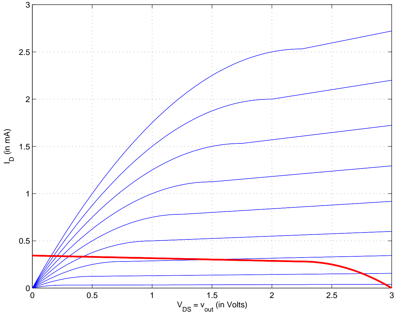
Problem 3, part (c): Early effect included
