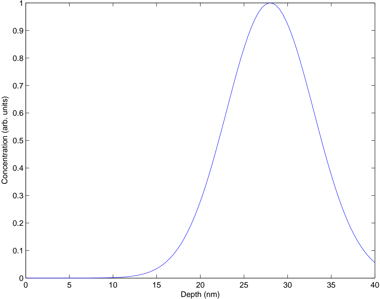
Problem 1b: Implanting 30keV P into Si through 15nm-thick oxide.
