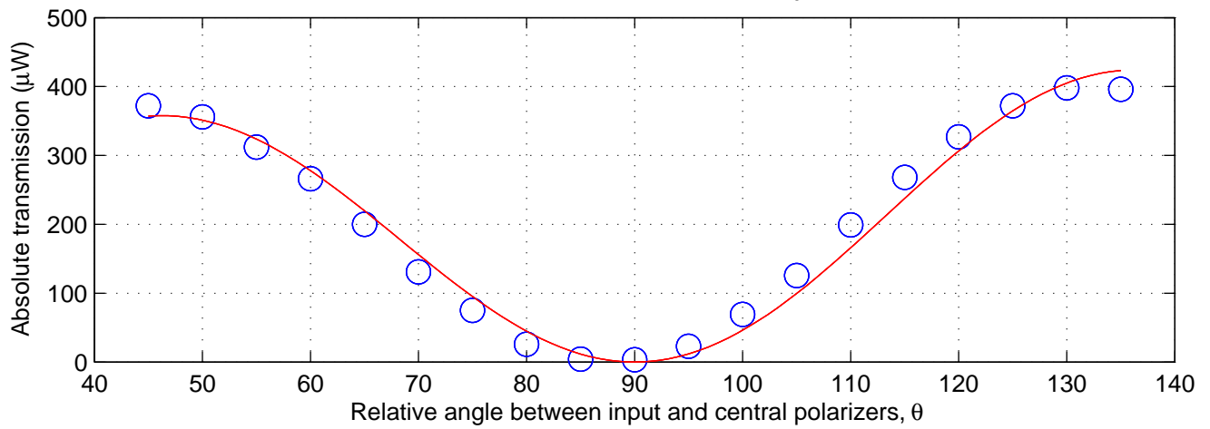
Measured data and fitted curve with \theta_0 = 92.4^\circ
