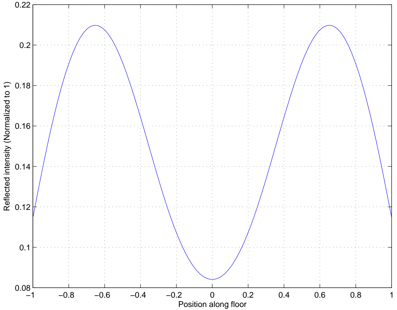
Haidinger fringe from a perfectly flat slide
