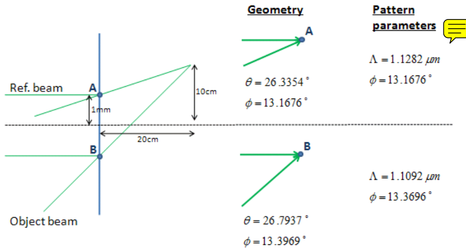
Figure 3: Characterization of the hologram interference pattern in terms of \Lambda and \phi parameters. For simplicity, we analyze only the endpoints A and B, and invoke the plane wave approximation.
