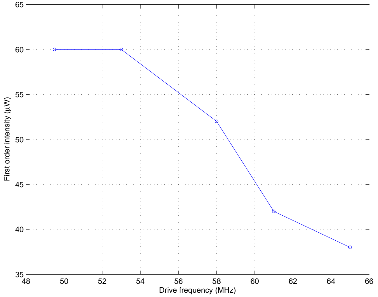
Diffraction efficiency vs. frequency
